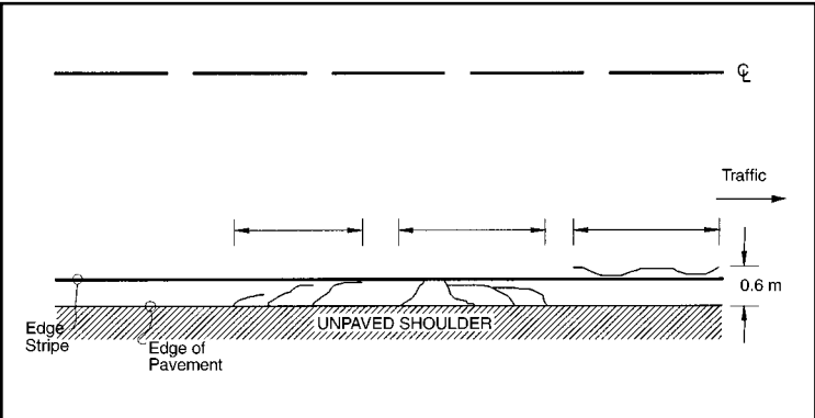
FIGURE 11 Distress Type ACP 3—Edge Cracking
